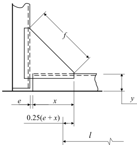
Fig. III 1-5 Bracket
