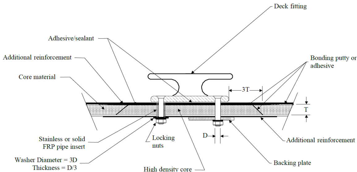
Fig. III 2-26 Deck Fittings
