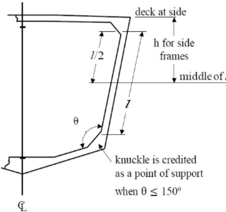
Fig. III 2-13 Transverse Side Frame
