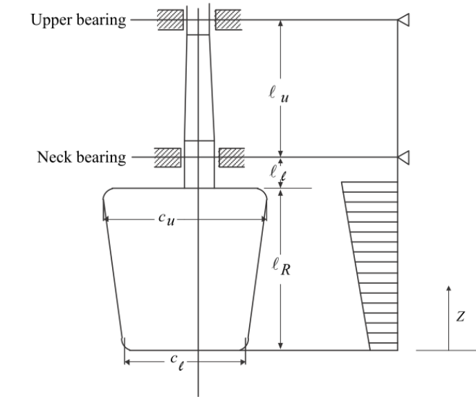
(a) Regular Spade Rudder
