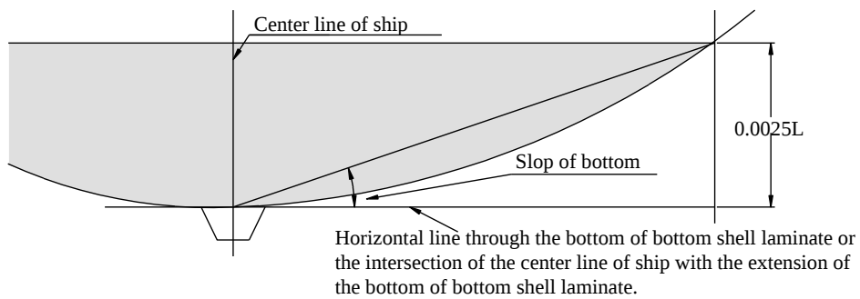
Fig. II 3-4 Slope of Bottom
