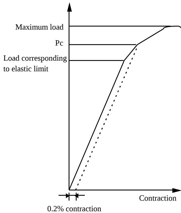
Fig. I 2-8 Load-Contraction Diagram
