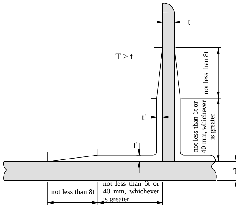
Fig. I 5-1A Dimensions of Overlap of T-Joints
