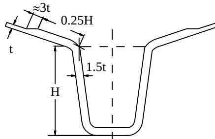
Fig. II 3-2 Vertical Keels and Slegs
